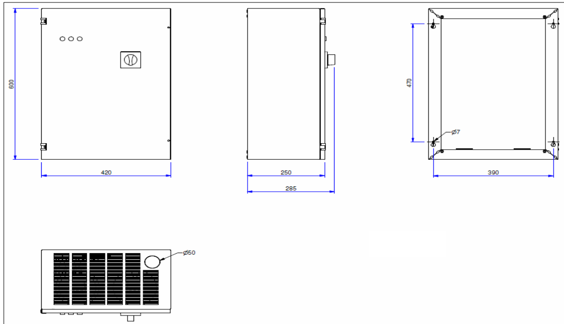
Cabina 1 / Enclosure 1
