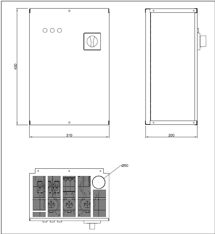
Cabina 1 / Enclosure 1
