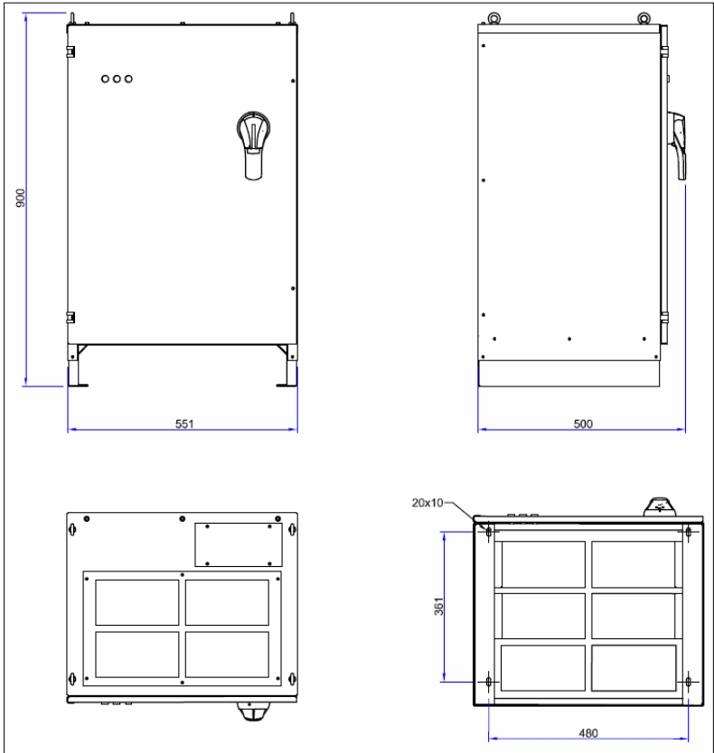
Cabina 2 / Enclosure 2
