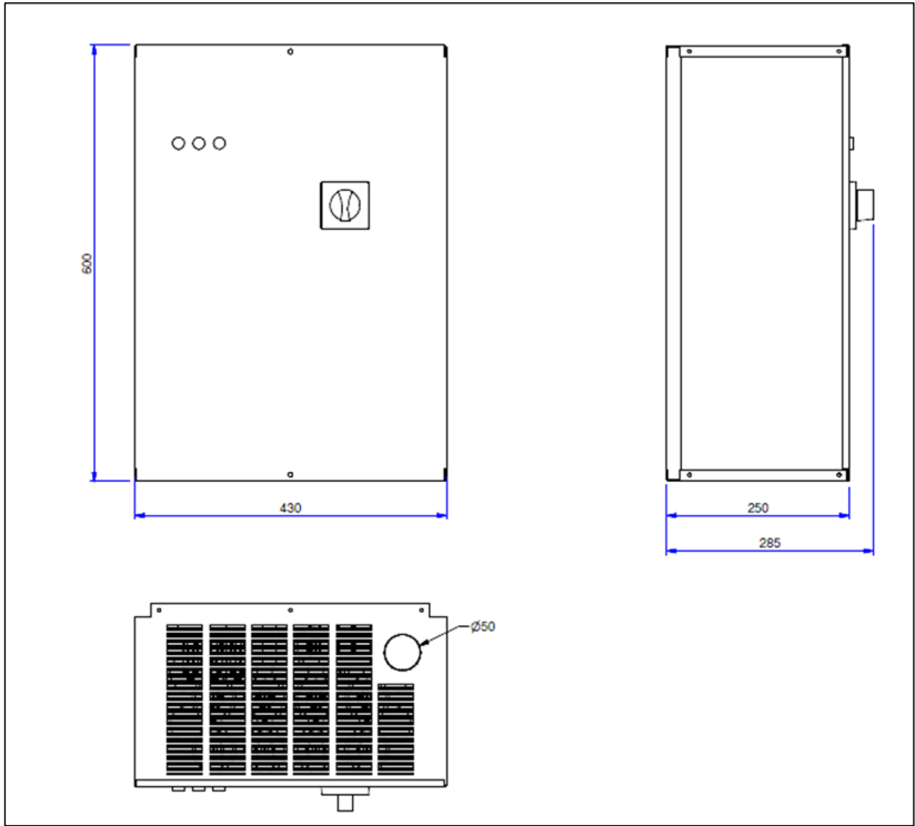
Cabina 3 / Enclosure 3
